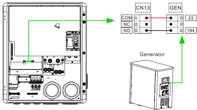
Communication connection between SYN 200-XH-US and Generator
